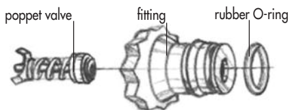
DISASSEMBLED FITTING
